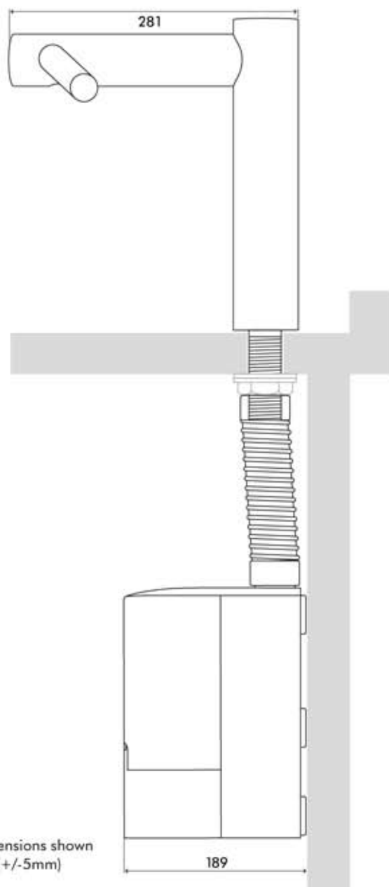
SIDE ELEVATION
